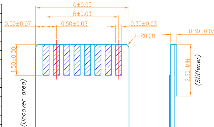
Recommended FPC/FFC Dimensions
