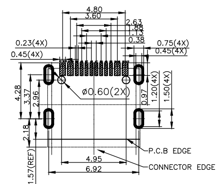
RECOMMENDED P.C.B. LAYOUT (T:0.80mm)
