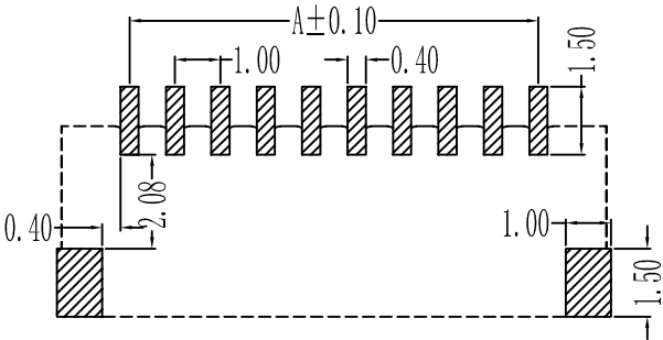
PCB Layout
