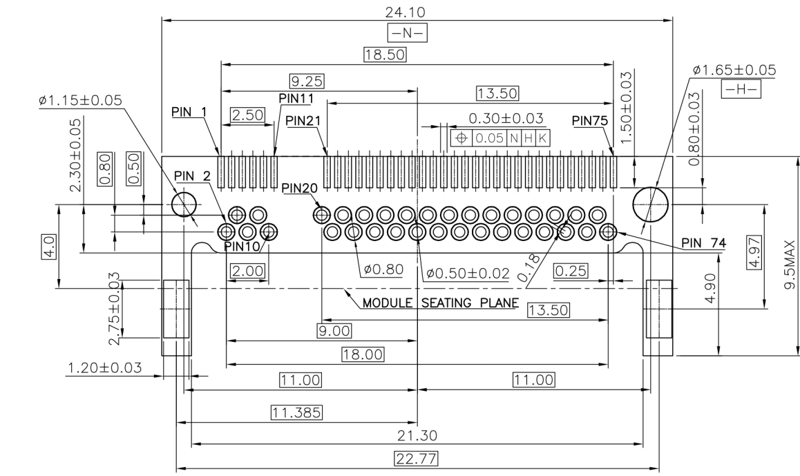
RECOMMENDED PCB LAYOUT DEFAULT TOLERANCE ±0.05MM
