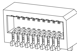
3D VIEW
