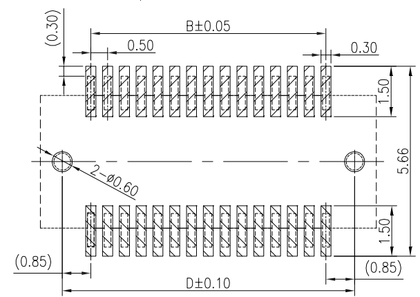
RECOMMENDED PCB PATTERN DIM.
